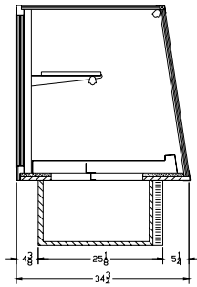
END VIEW
